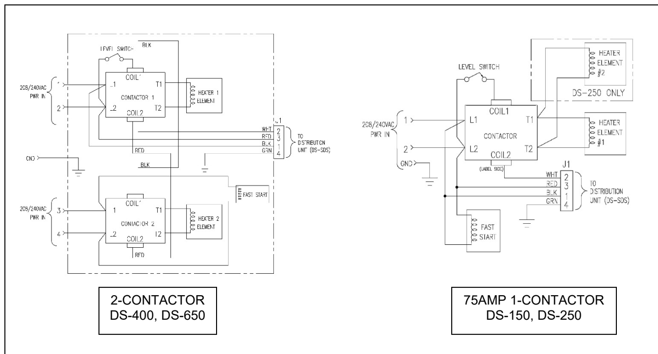
Figure 4 Wiring diagram
