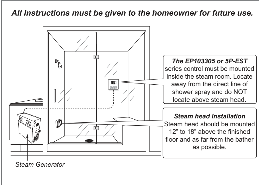
Figure 4 - Installation Suggestions
