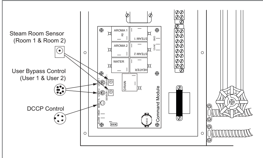
Figure 7 - Circuit Board Connections
