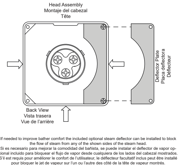
Figure 12 - Optional Deflector
