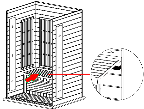
FIG 10 Installing Bench
