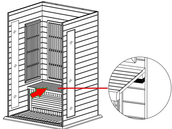
FIG 10 Installing Bench
