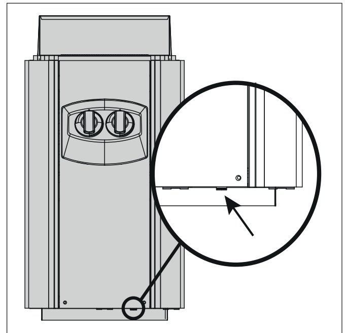
Figure 8. Reset button for overheat protector
