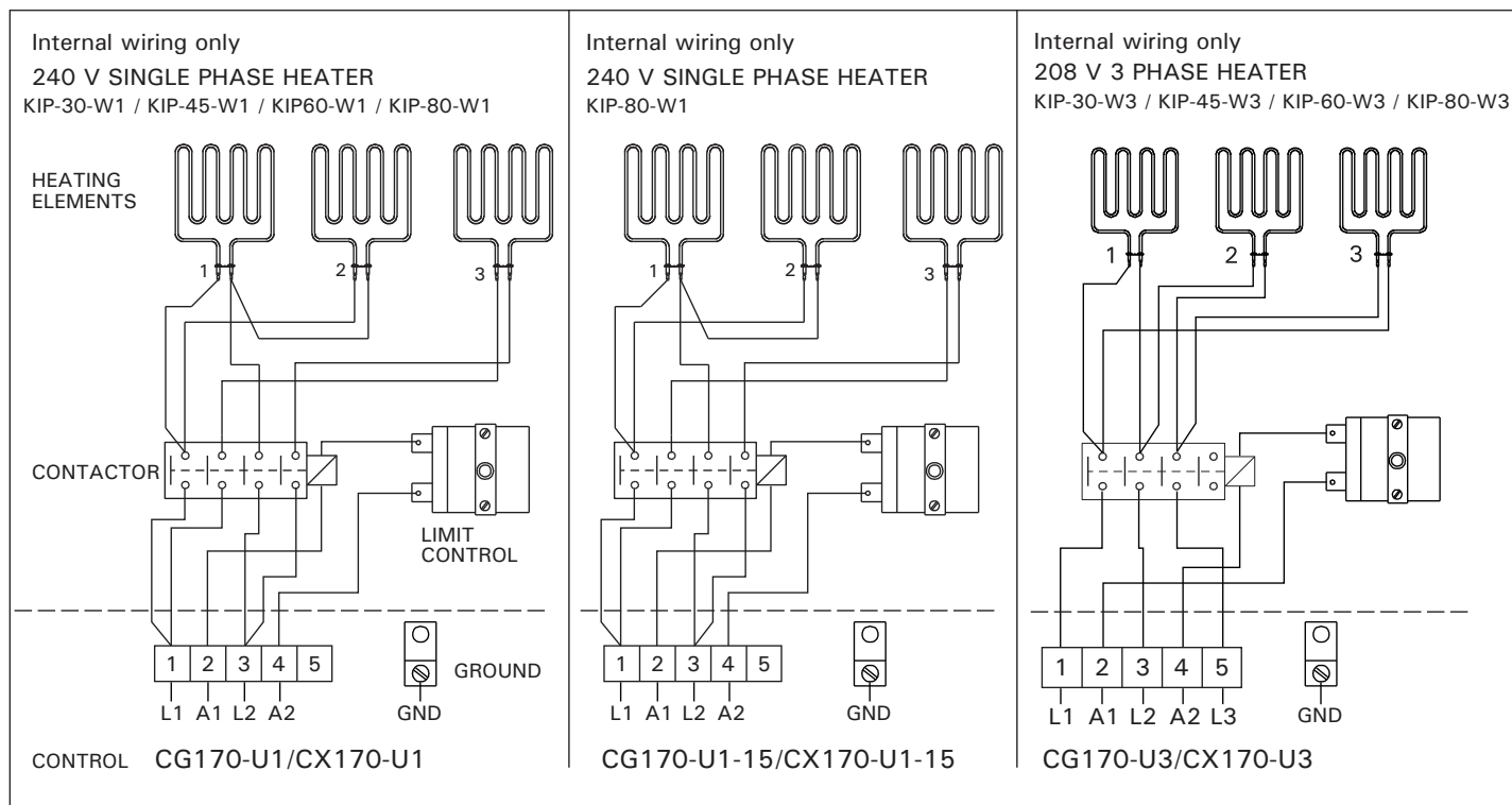
Figure 6. Wiring diagram
